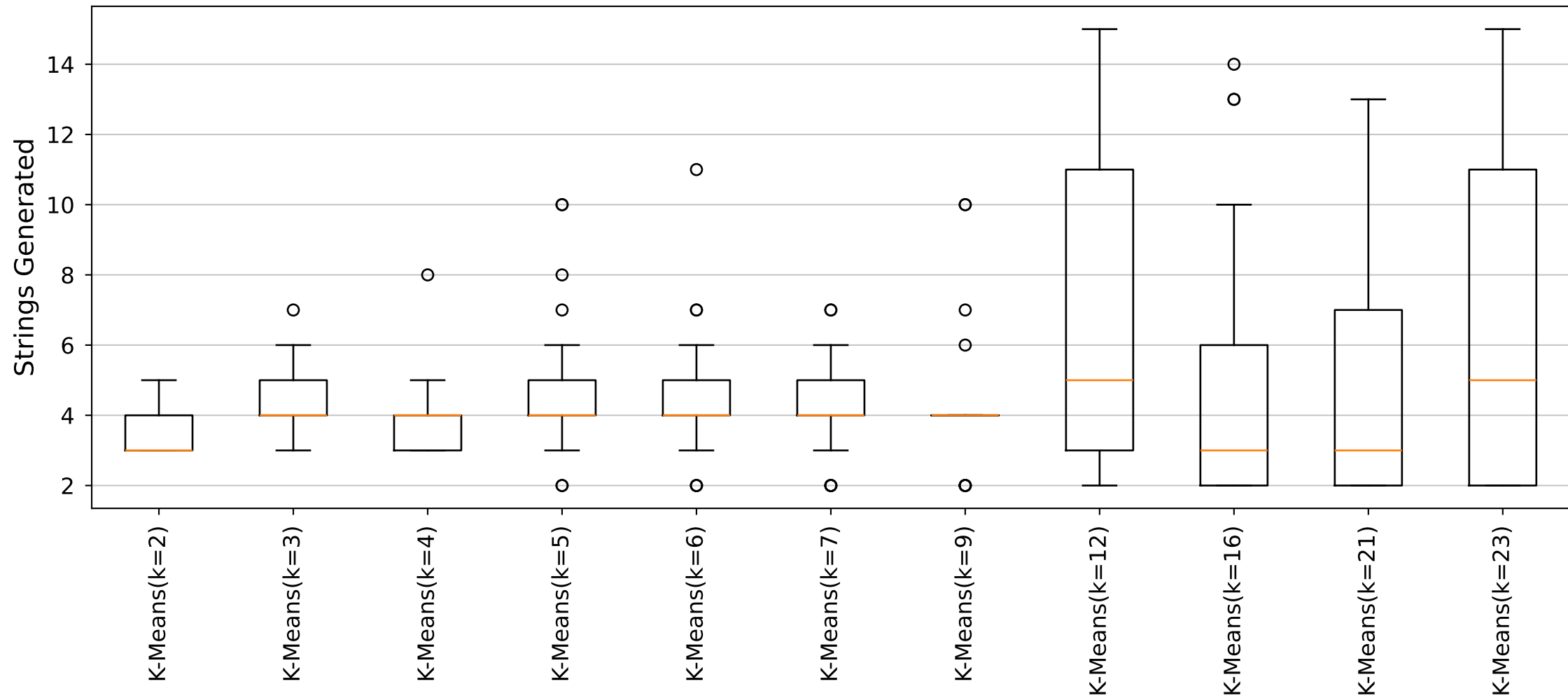
YARA Rules Strings Generated Distribution (Cluster6_Size23 dataset)
